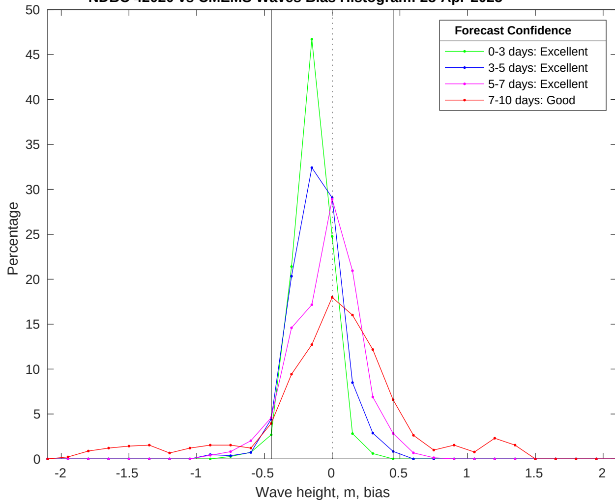
NDBC 42020 vs CMEMS Waves Bias Histogram: 28-Apr-2025
