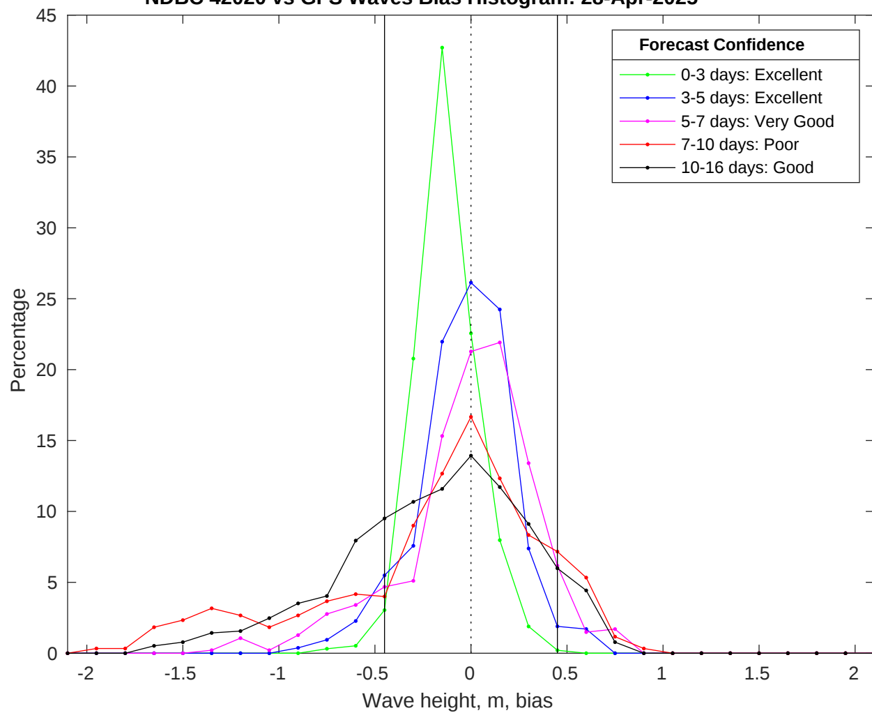
NDBC 42020 vs GFS Waves Bias Histogram: 28-Apr-2025
