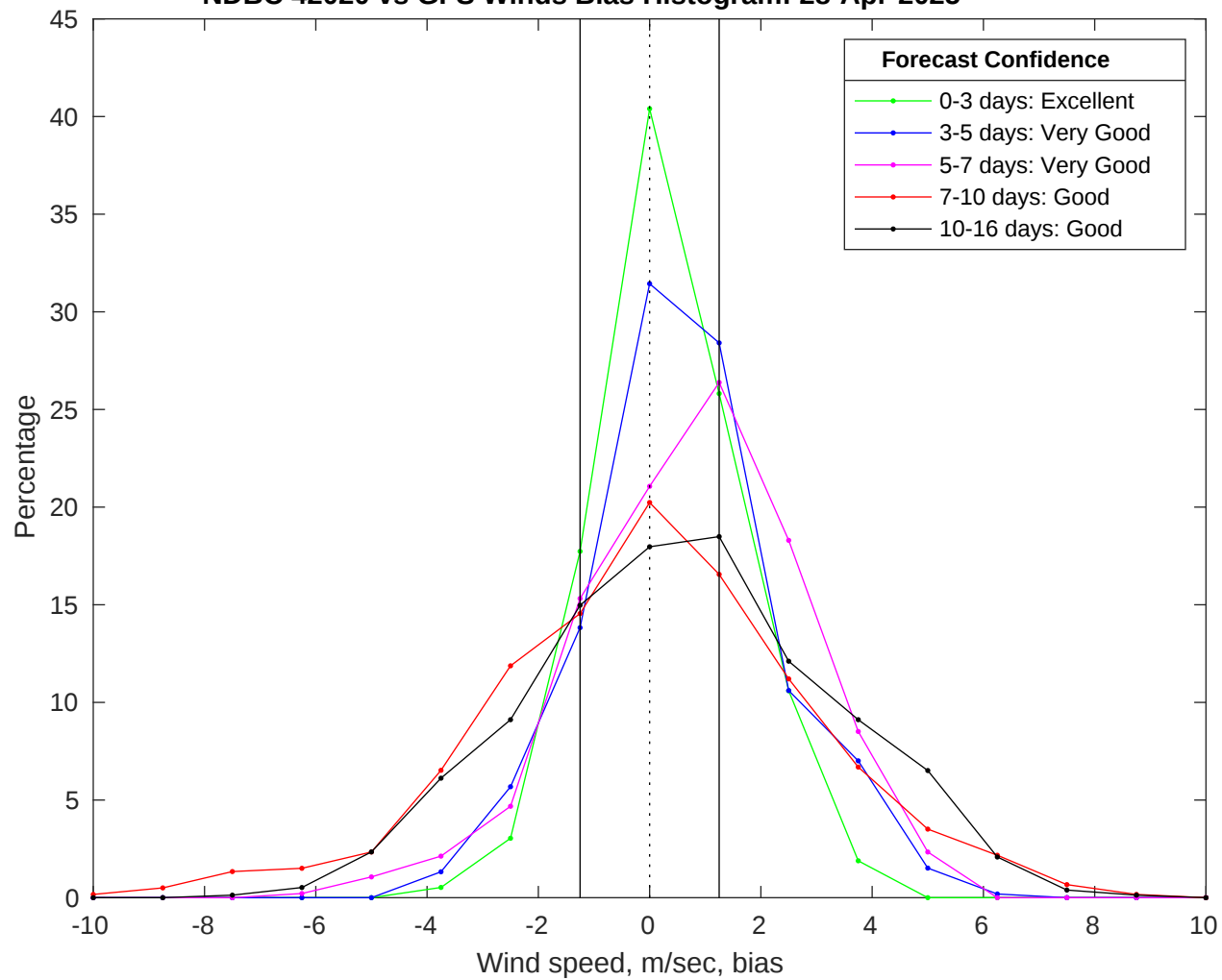
NDBC 42020 vs GFS Winds Bias Histogram: 28-Apr-2025
