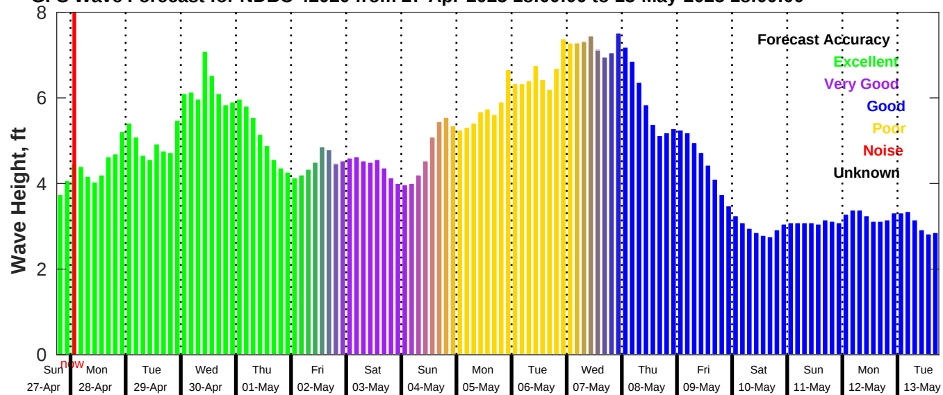
GFS Wave Forecast for NDBC 42020 from 27-Apr-2025 18:00:00 to 13-May-2025 18:00:00
