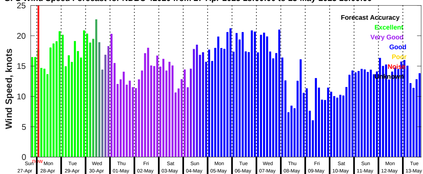
GFS Wind Speed Forecast for NDBC 42020 from 27-Apr-2025 18:00:00 to 13-May-2025 18:00:00
