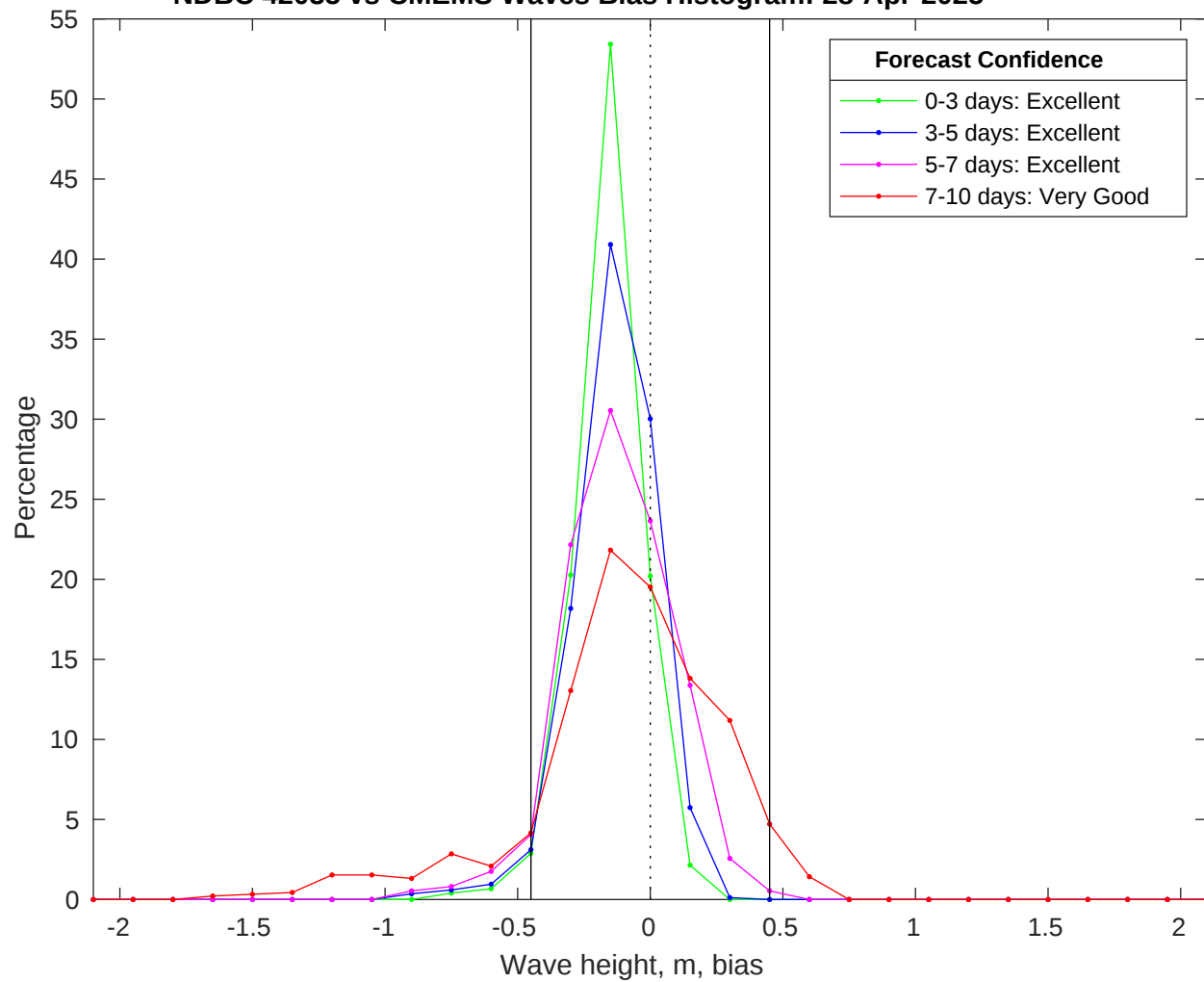
NDBC 42035 vs CMEMS Waves Bias Histogram: 28-Apr-2025
