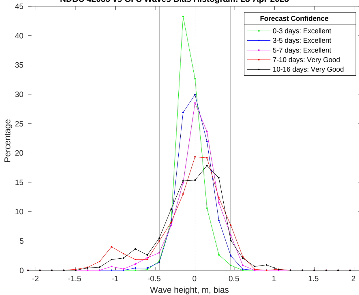
NDBC 42035 vs GFS Waves Bias Histogram: 28-Apr-2025
