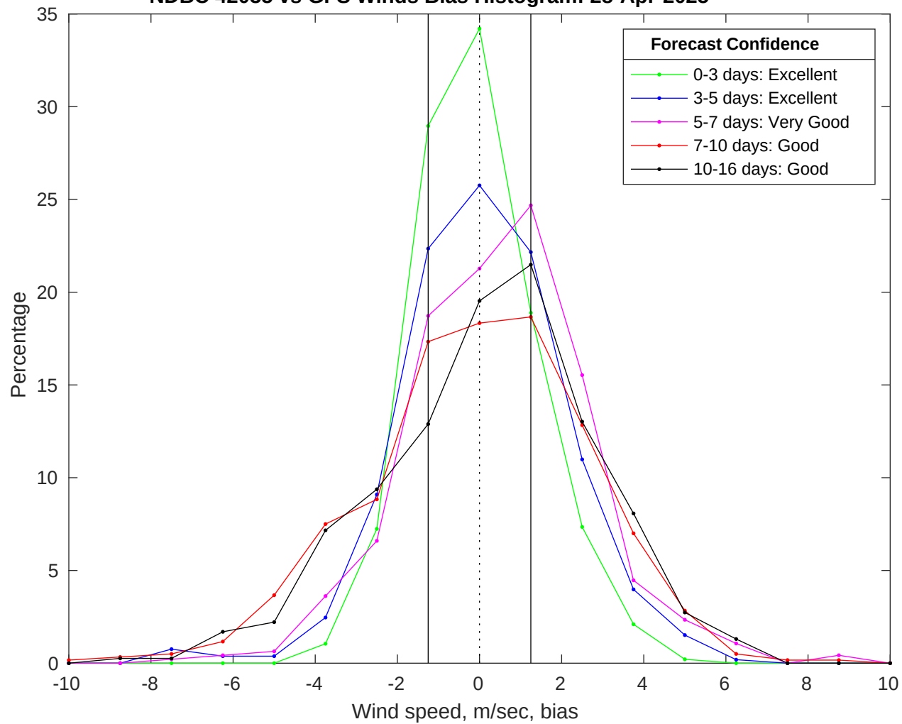
NDBC 42035 vs GFS Winds Bias Histogram: 28-Apr-2025
