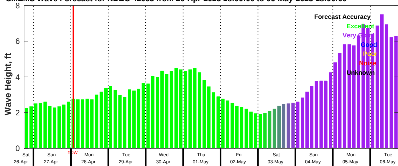
CMEMS Wave Forecast for NDBC 42035 from 26-Apr-2025 18:00:00 to 06-May-2025 18:00:00
