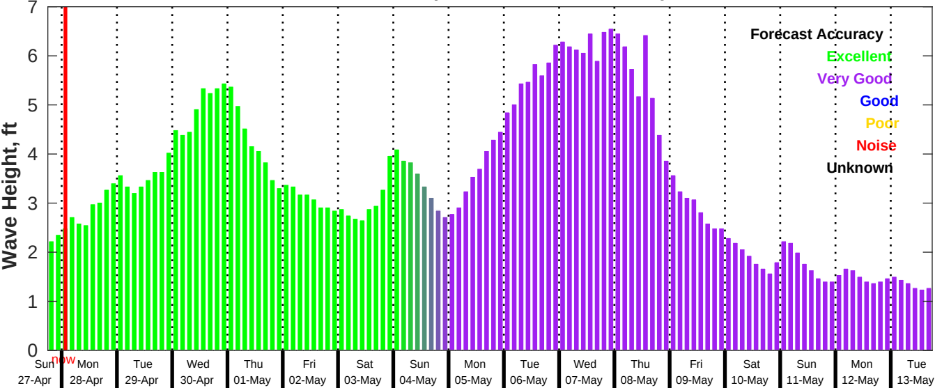
GFS Wave Forecast for NDBC 42035 from 27-Apr-2025 18:00:00 to 13-May-2025 18:00:00
