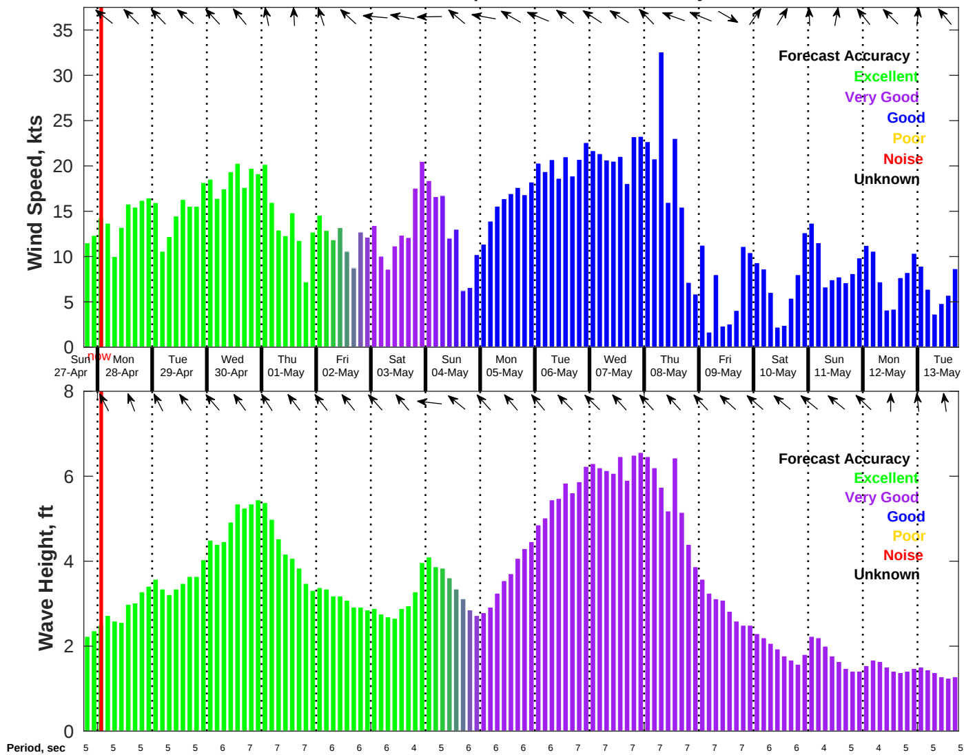
Wind & Wave Forecast for NDBC 42035 from 27-Apr-2025 18:00:00 to 13-May-2025 18:00:00
