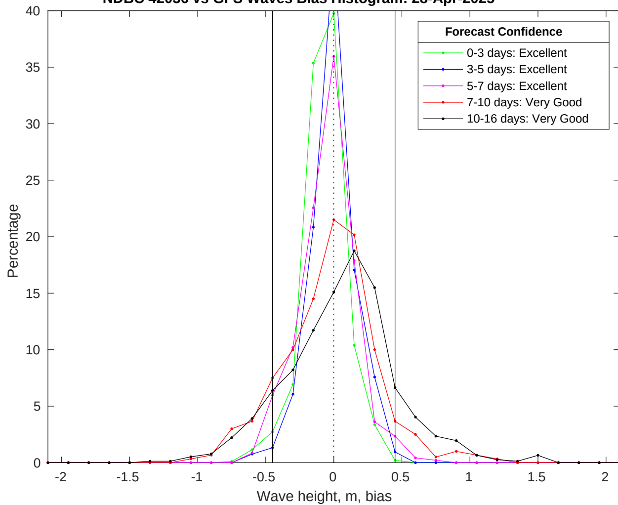
NDBC 42036 vs GFS Waves Bias Histogram: 28-Apr-2025
