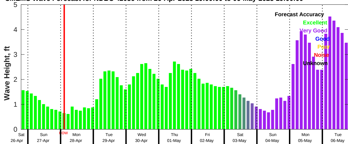
CMEMS Wave Forecast for NDBC 42036 from 26-Apr-2025 19:00:00 to 06-May-2025 19:00:00
