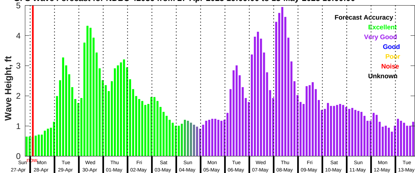
GFS Wave Forecast for NDBC 42036 from 27-Apr-2025 19:00:00 to 13-May-2025 19:00:00
