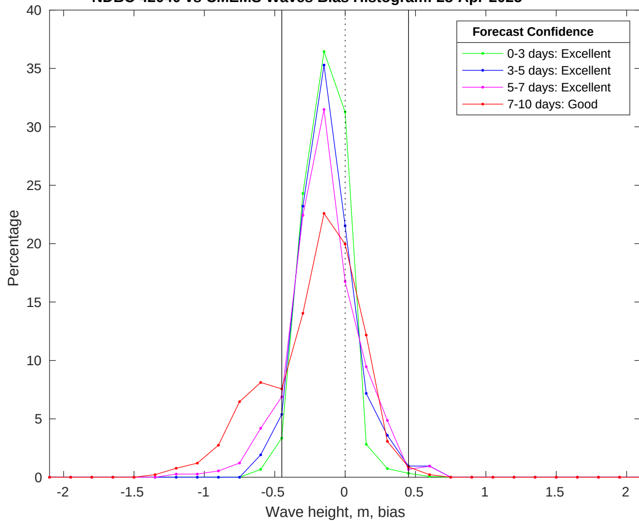
NDBC 42040 vs CMEMS Waves Bias Histogram: 28-Apr-2025
