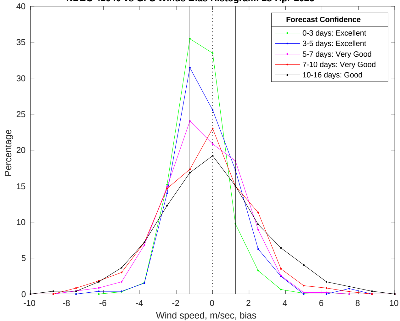
NDBC 42040 vs GFS Winds Bias Histogram: 28-Apr-2025
