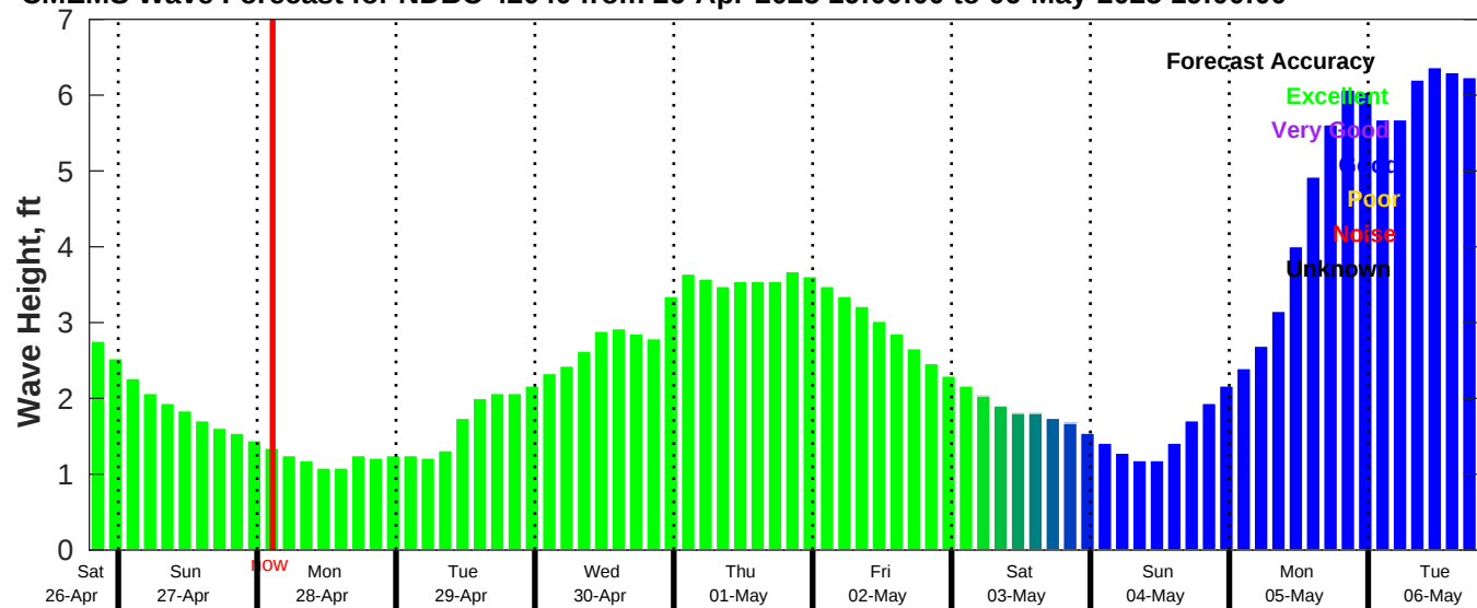
CMEMS Wave Forecast for NDBC 42040 from 26-Apr-2025 19:00:00 to 06-May-2025 19:00:00
