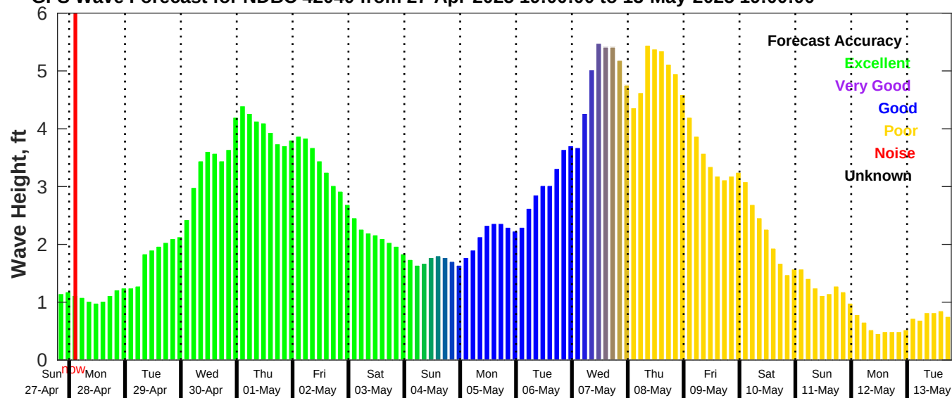
GFS Wave Forecast for NDBC 42040 from 27-Apr-2025 19:00:00 to 13-May-2025 19:00:00
