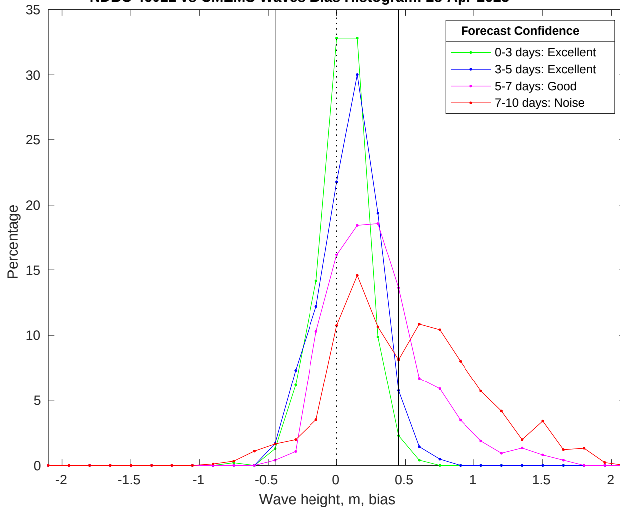
NDBC 46011 vs CMEMS Waves Bias Histogram: 28-Apr-2025
