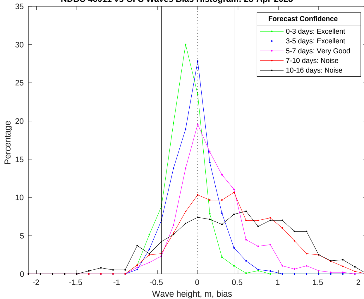
NDBC 46011 vs GFS Waves Bias Histogram: 28-Apr-2025
