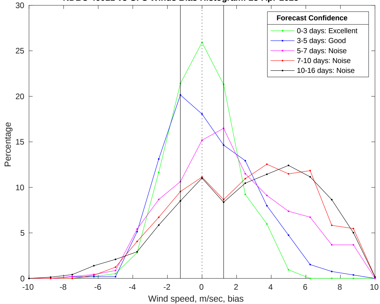
NDBC 46011 vs GFS Winds Bias Histogram: 28-Apr-2025
