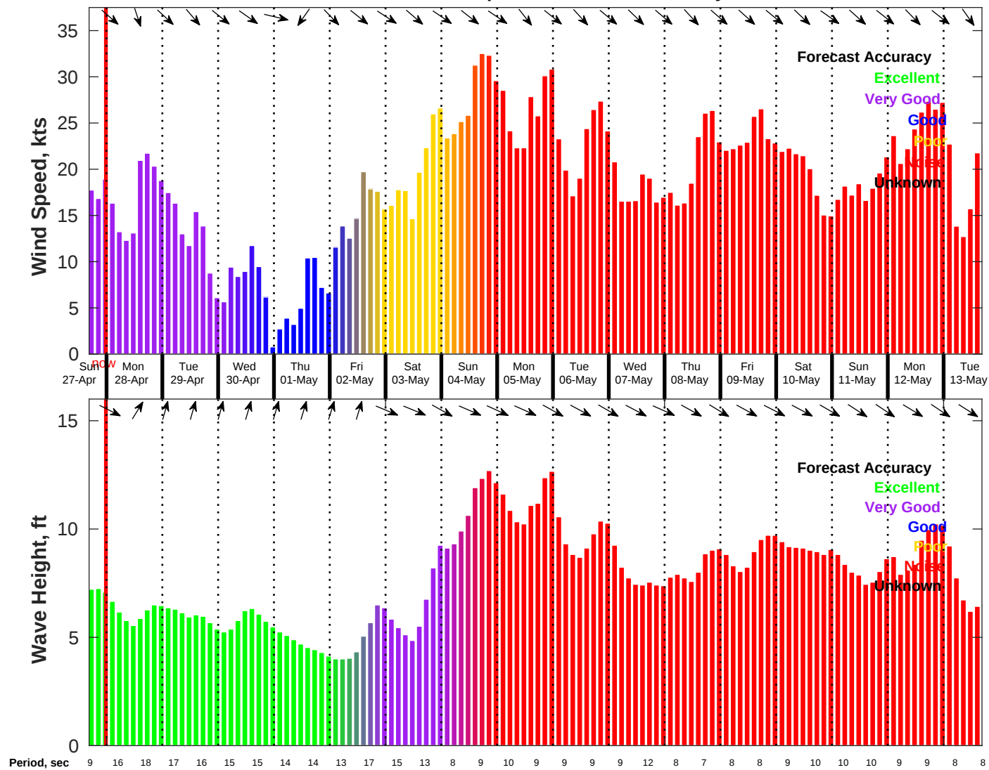
Wind & Wave Forecast for NDBC 46011 from 27-Apr-2025 16:00:00 to 13-May-2025 16:00:00
