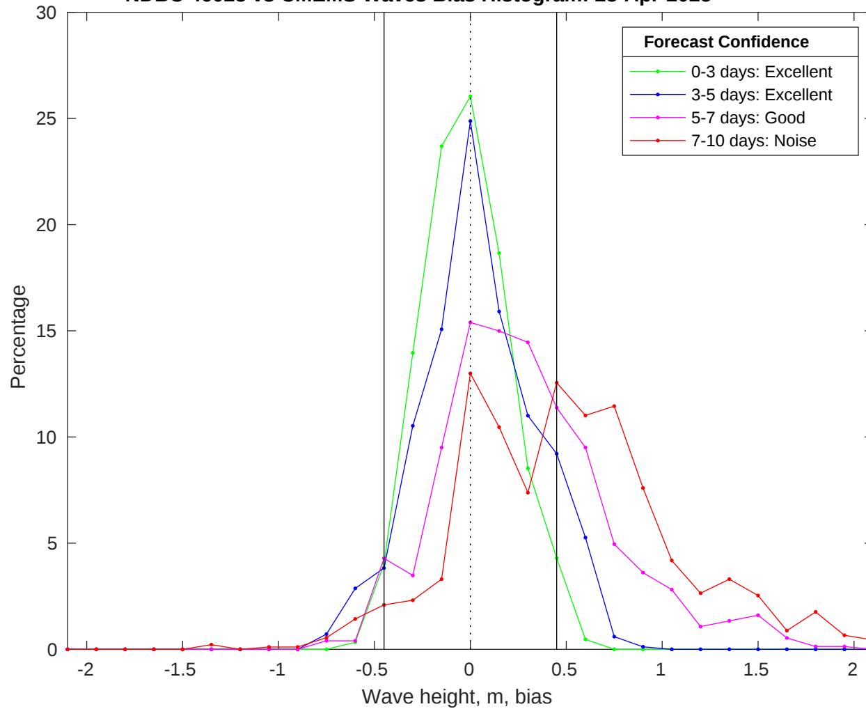
NDBC 46028 vs CMEMS Waves Bias Histogram: 28-Apr-2025
