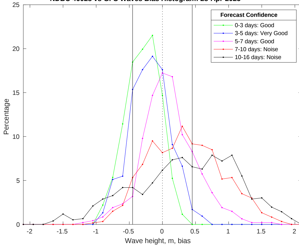
NDBC 46028 vs GFS Waves Bias Histogram: 28-Apr-2025
