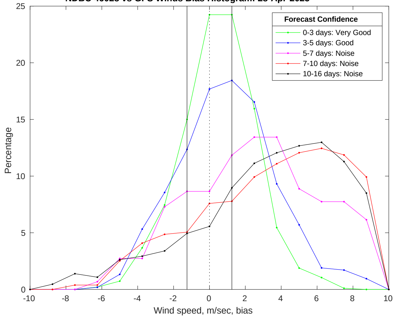
NDBC 46028 vs GFS Winds Bias Histogram: 28-Apr-2025
