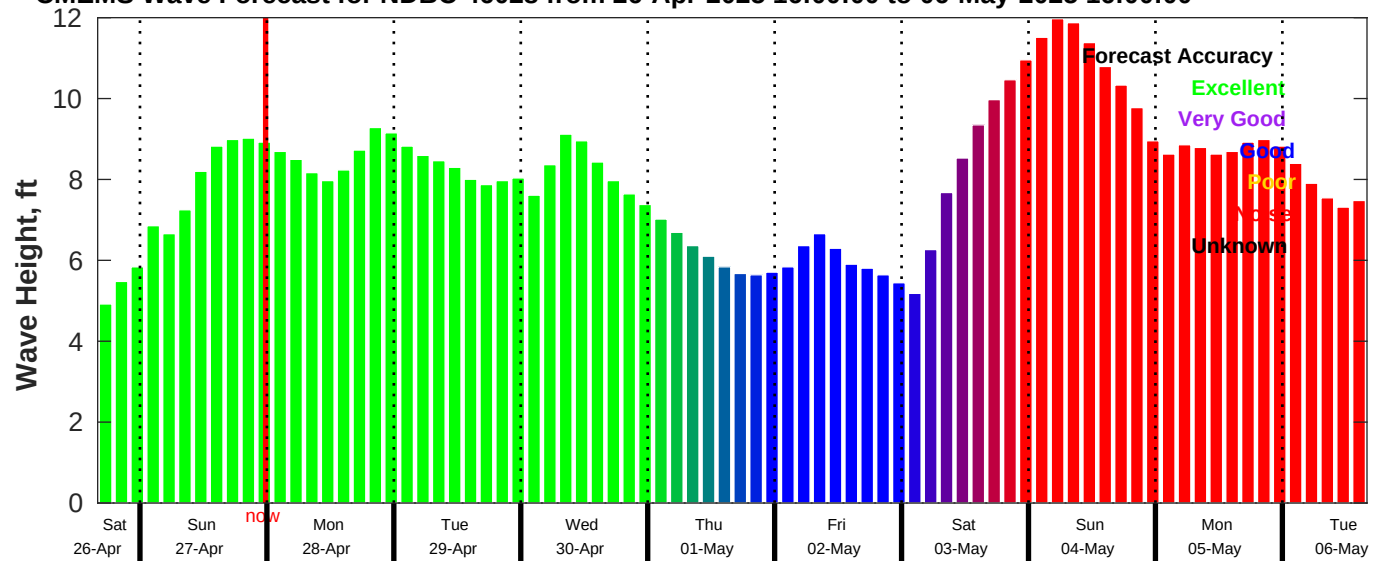
CMEMS Wave Forecast for NDBC 46028 from 26-Apr-2025 16:00:00 to 06-May-2025 16:00:00
