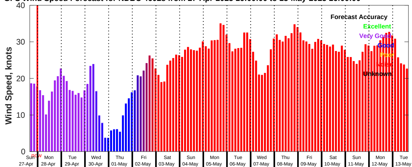
GFS Wind Speed Forecast for NDBC 46028 from 27-Apr-2025 16:00:00 to 13-May-2025 16:00:00
