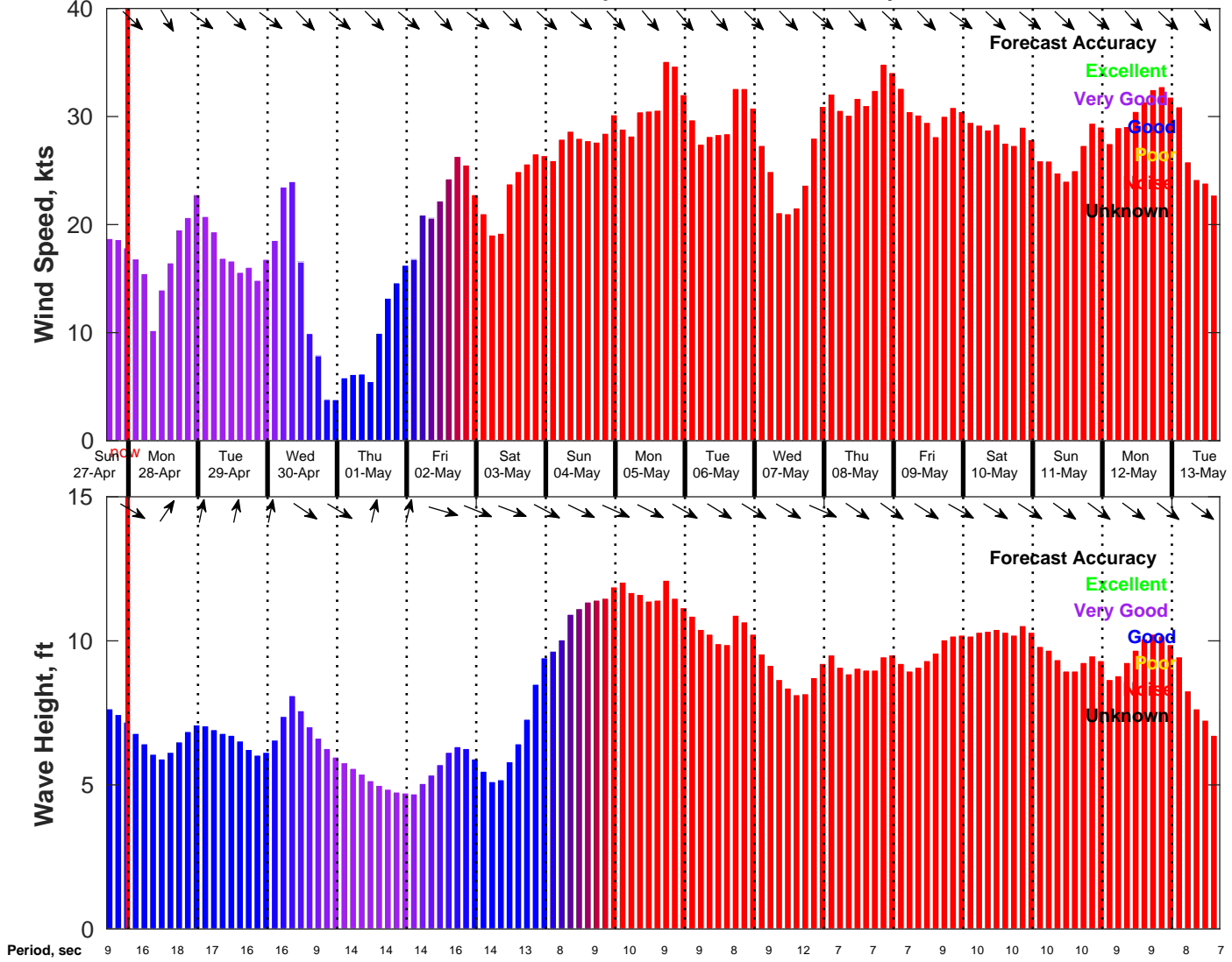
Wind & Wave Forecast for NDBC 46028 from 27-Apr-2025 16:00:00 to 13-May-2025 16:00:00
