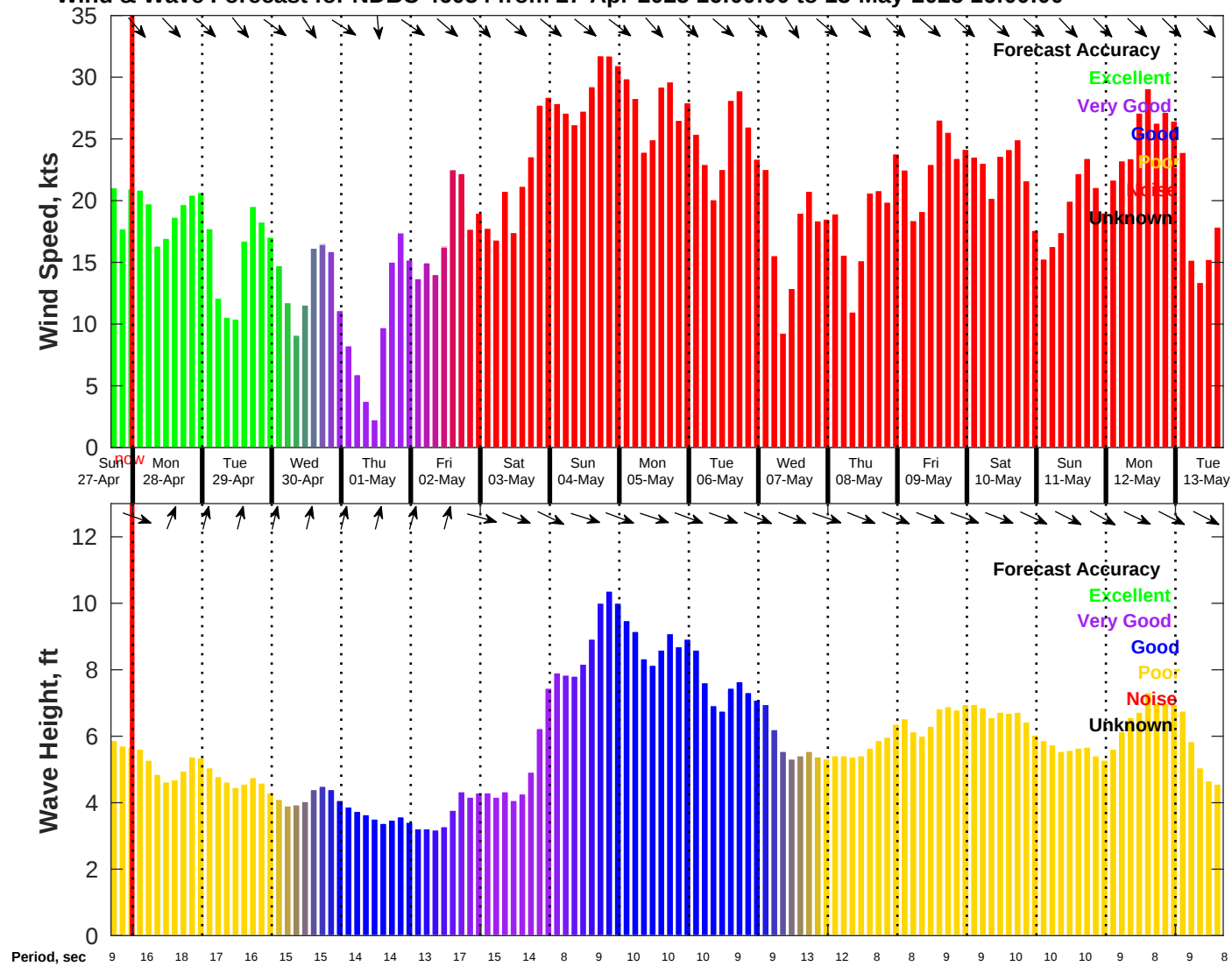
Wind & Wave Forecast for NDBC 46054 from 27-Apr-2025 16:00:00 to 13-May-2025 16:00:00
