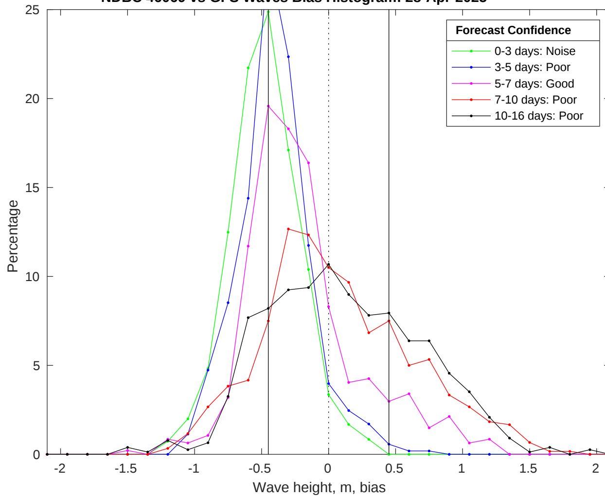
NDBC 46069 vs GFS Waves Bias Histogram: 28-Apr-2025
