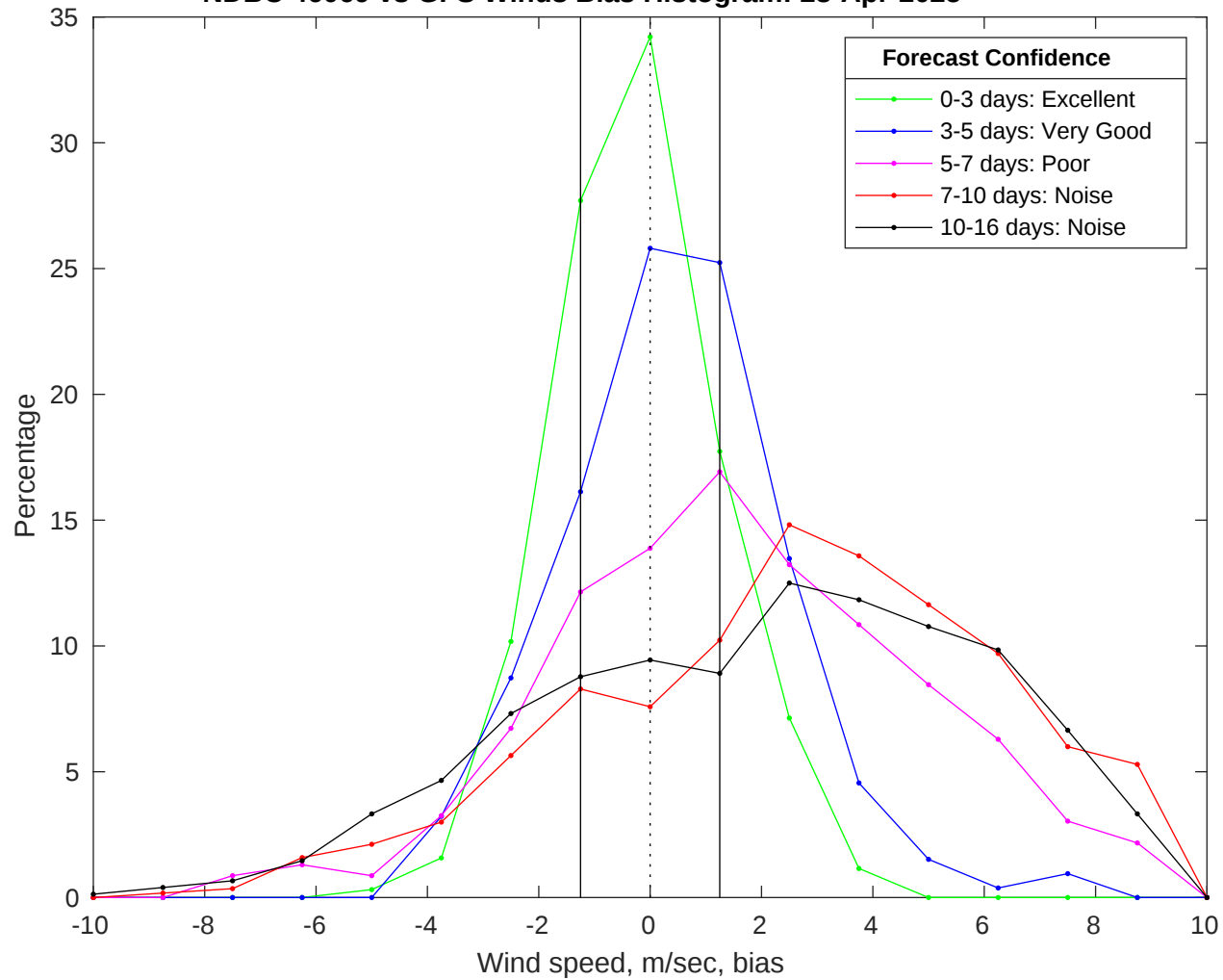
NDBC 46069 vs GFS Winds Bias Histogram: 28-Apr-2025
