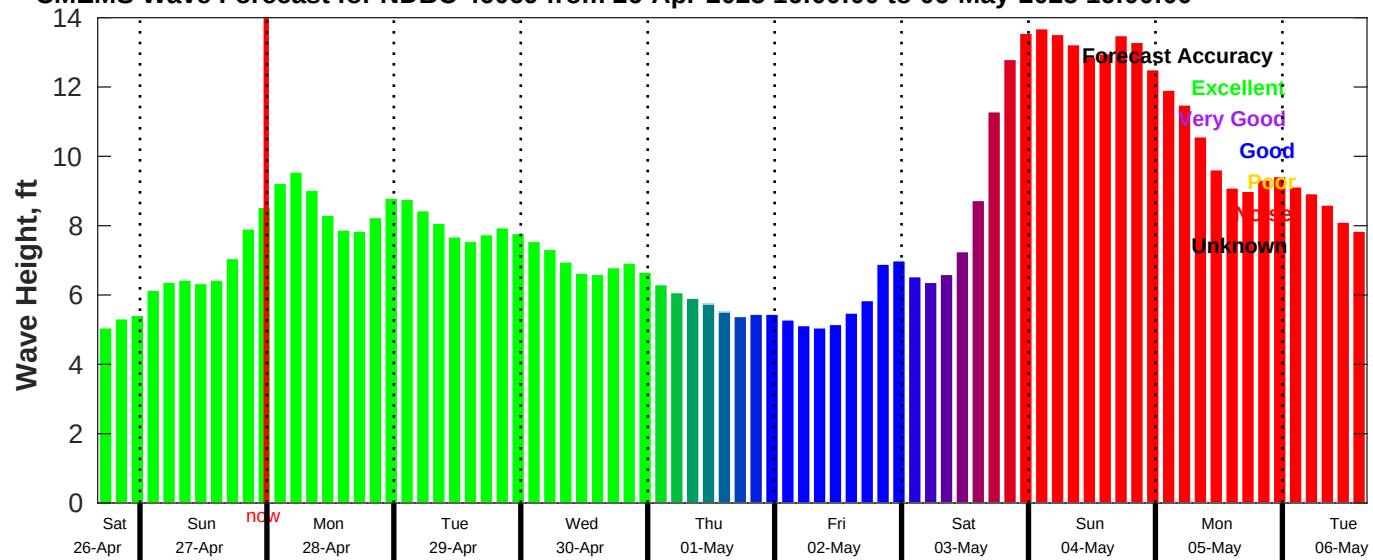
CMEMS Wave Forecast for NDBC 46069 from 26-Apr-2025 16:00:00 to 06-May-2025 16:00:00
