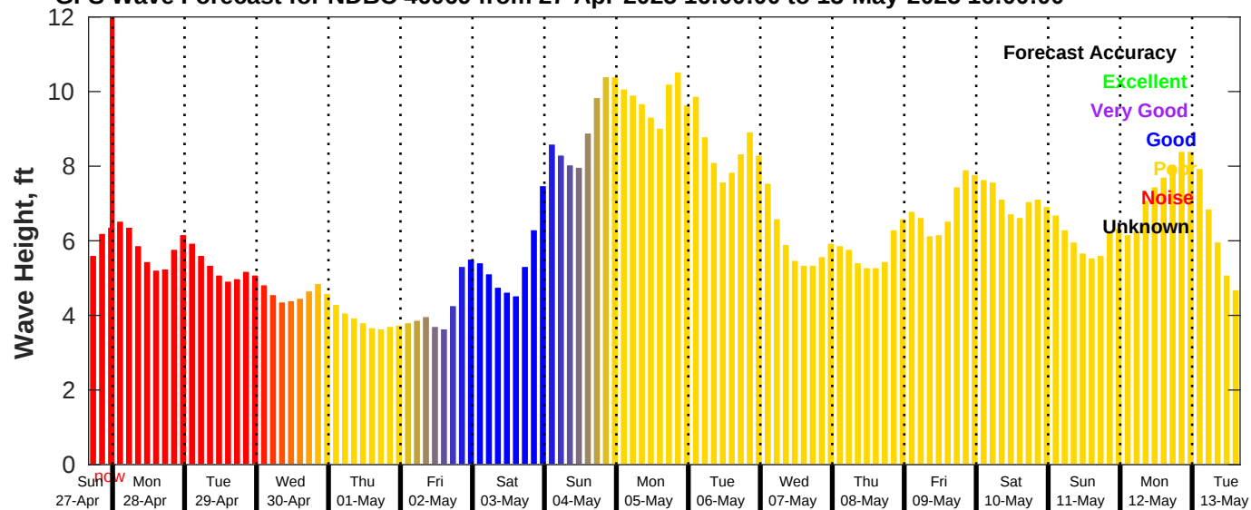
GFS Wave Forecast for NDBC 46069 from 27-Apr-2025 16:00:00 to 13-May-2025 16:00:00
