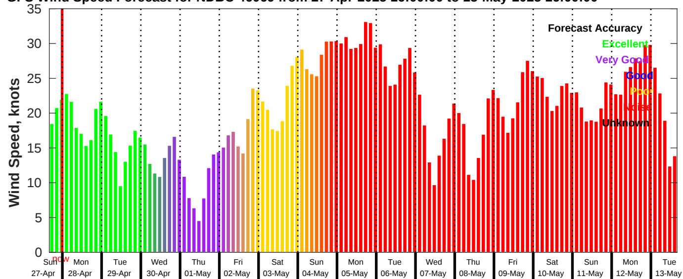
GFS Wind Speed Forecast for NDBC 46069 from 27-Apr-2025 16:00:00 to 13-May-2025 16:00:00
