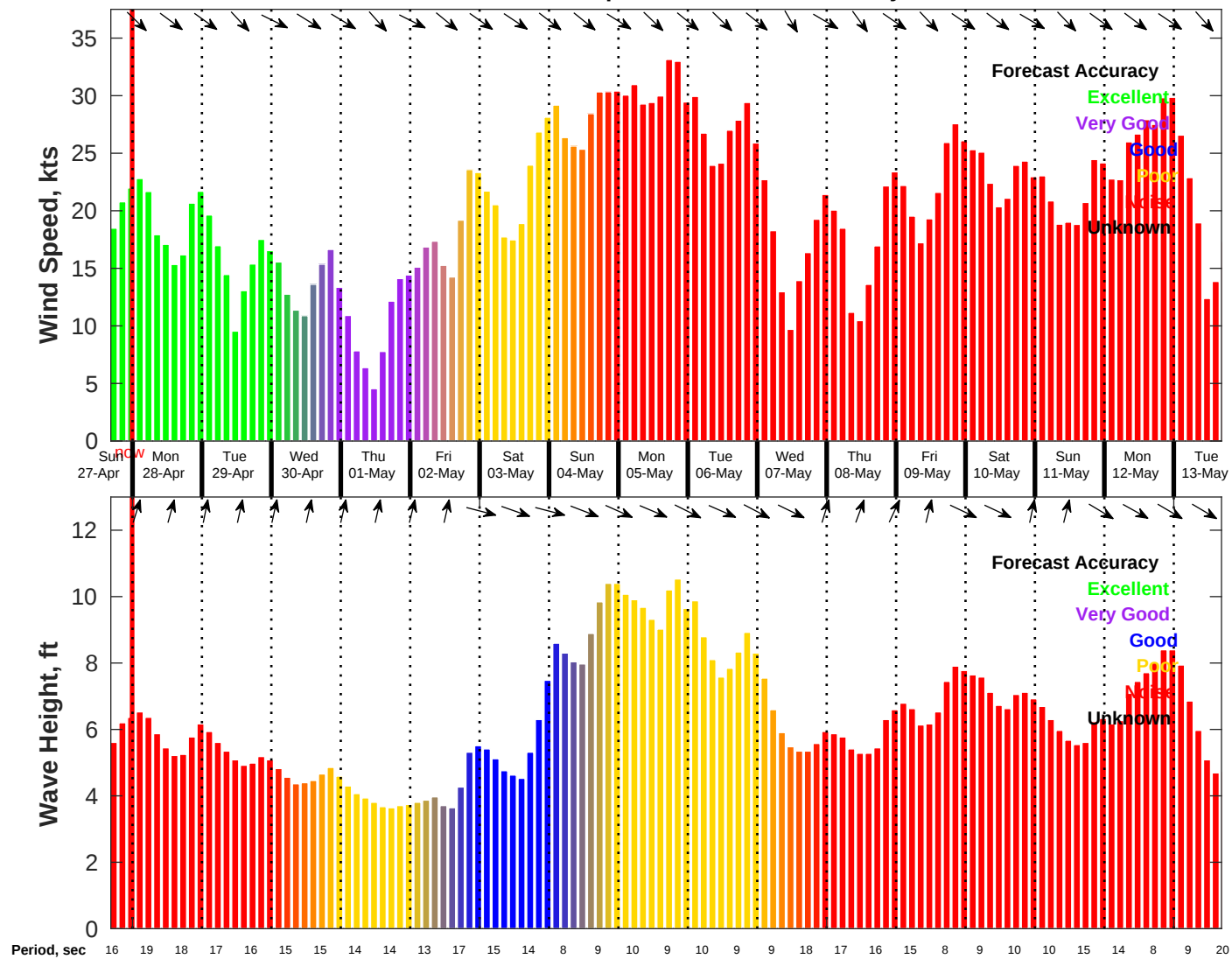
Wind & Wave Forecast for NDBC 46069 from 27-Apr-2025 16:00:00 to 13-May-2025 16:00:00
