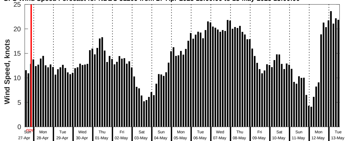
GFS Wind Speed Forecast for NDBC 51209 from 27-Apr-2025 13:00:00 to 13-May-2025 13:00:00
