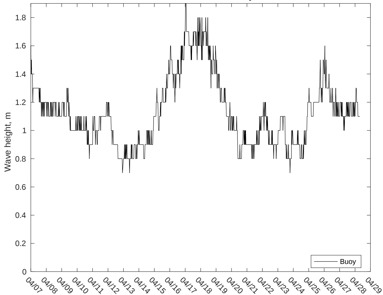
NDBC 52211 vs CMEMS Waves: 10 to 16 day forecast
