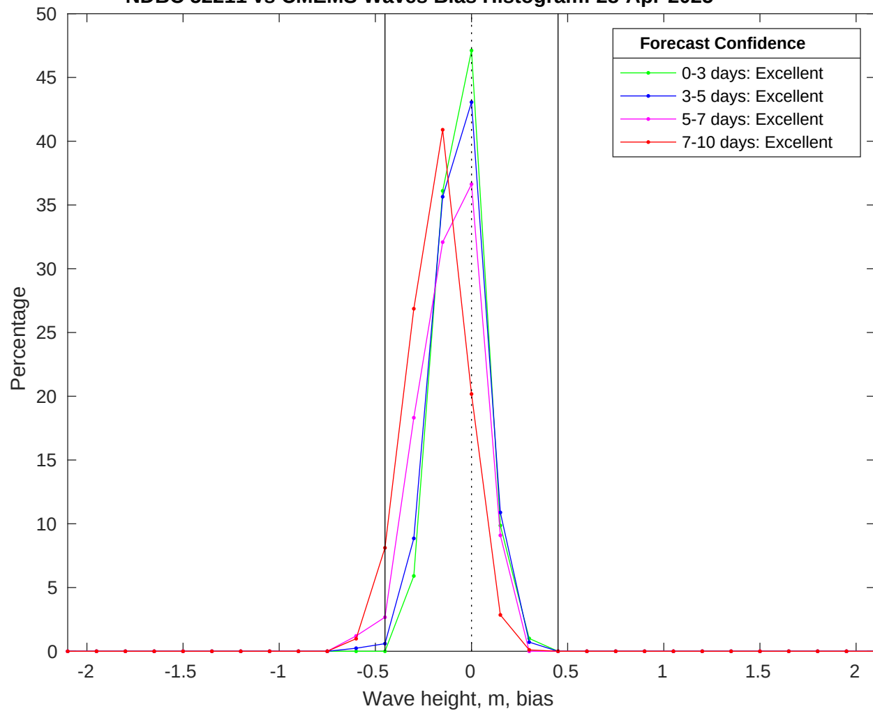
NDBC 52211 vs CMEMS Waves Bias Histogram: 28-Apr-2025
