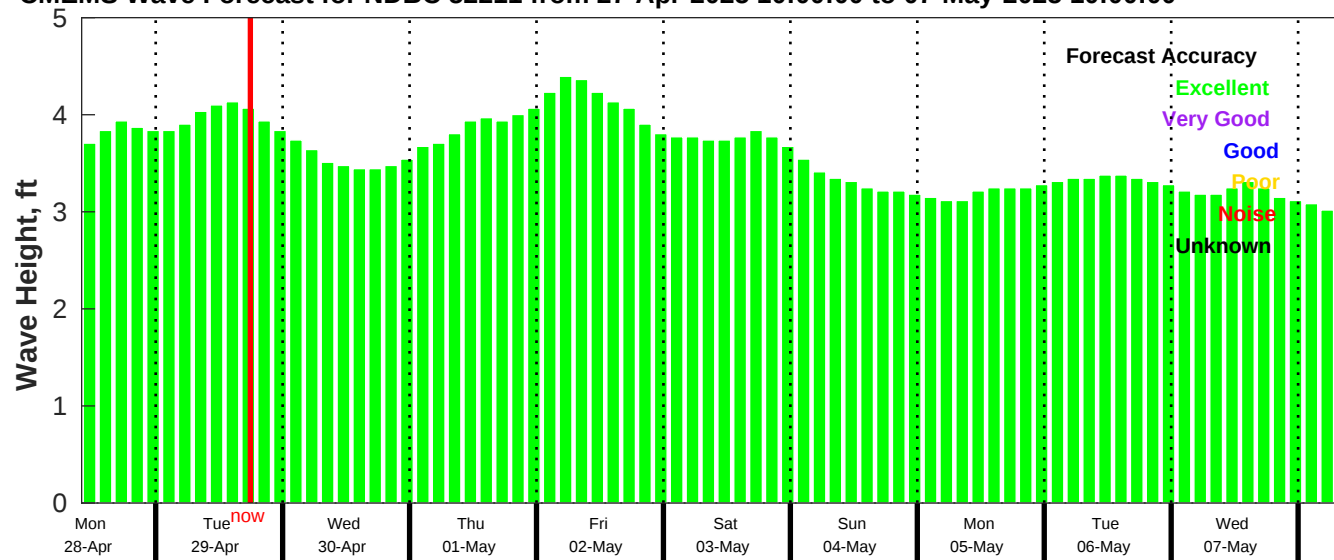
CMEMS Wave Forecast for NDBC 52211 from 27-Apr-2025 10:00:00 to 07-May-2025 10:00:00
