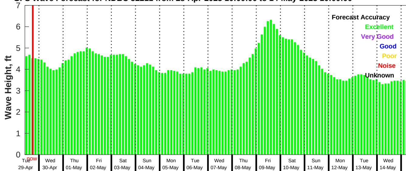
GFS Wave Forecast for NDBC 52211 from 28-Apr-2025 10:00:00 to 14-May-2025 10:00:00
