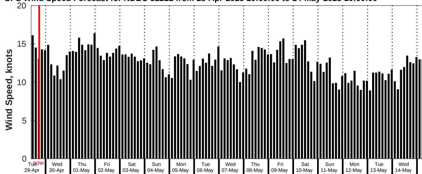
GFS Wind Speed Forecast for NDBC 52211 from 28-Apr-2025 10:00:00 to 14-May-2025 10:00:00
