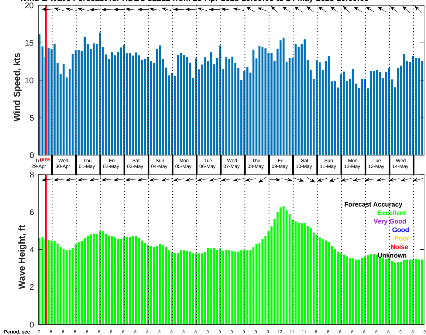
Wind & Wave Forecast for NDBC 52211 from 28-Apr-2025 10:00:00 to 14-May-2025 10:00:00
