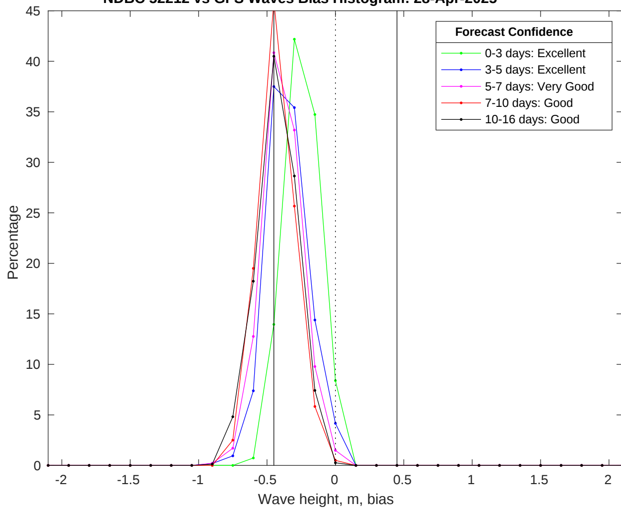
NDBC 52212 vs GFS Waves Bias Histogram: 28-Apr-2025
