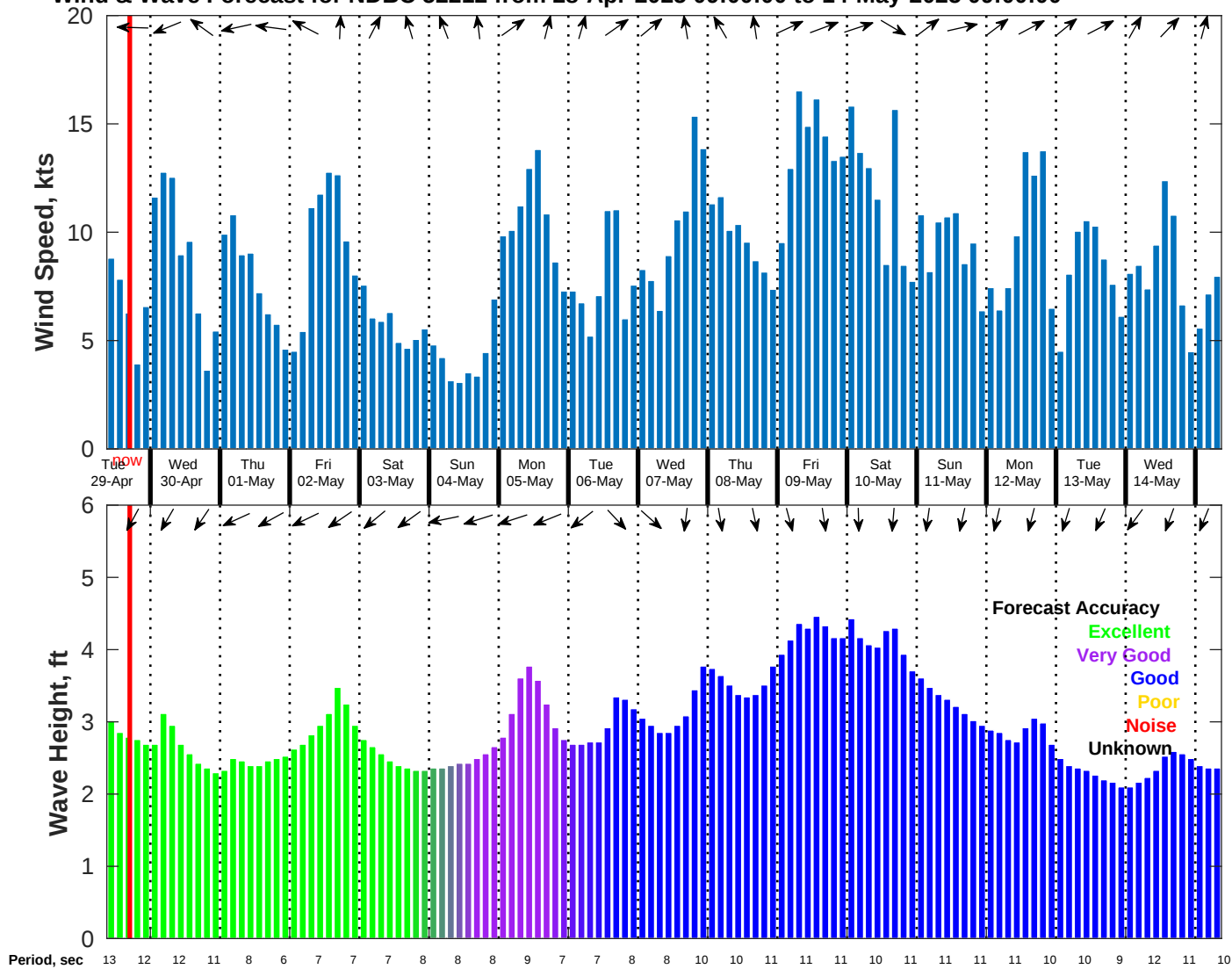
Wind & Wave Forecast for NDBC 52212 from 28-Apr-2025 09:00:00 to 14-May-2025 09:00:00
