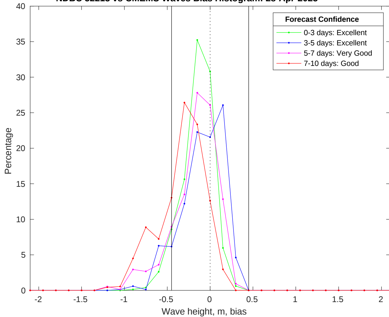
NDBC 52213 vs CMEMS Waves Bias Histogram: 28-Apr-2025
