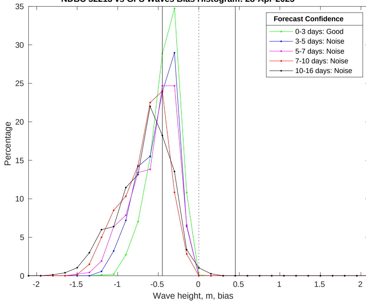
NDBC 52213 vs GFS Waves Bias Histogram: 28-Apr-2025
