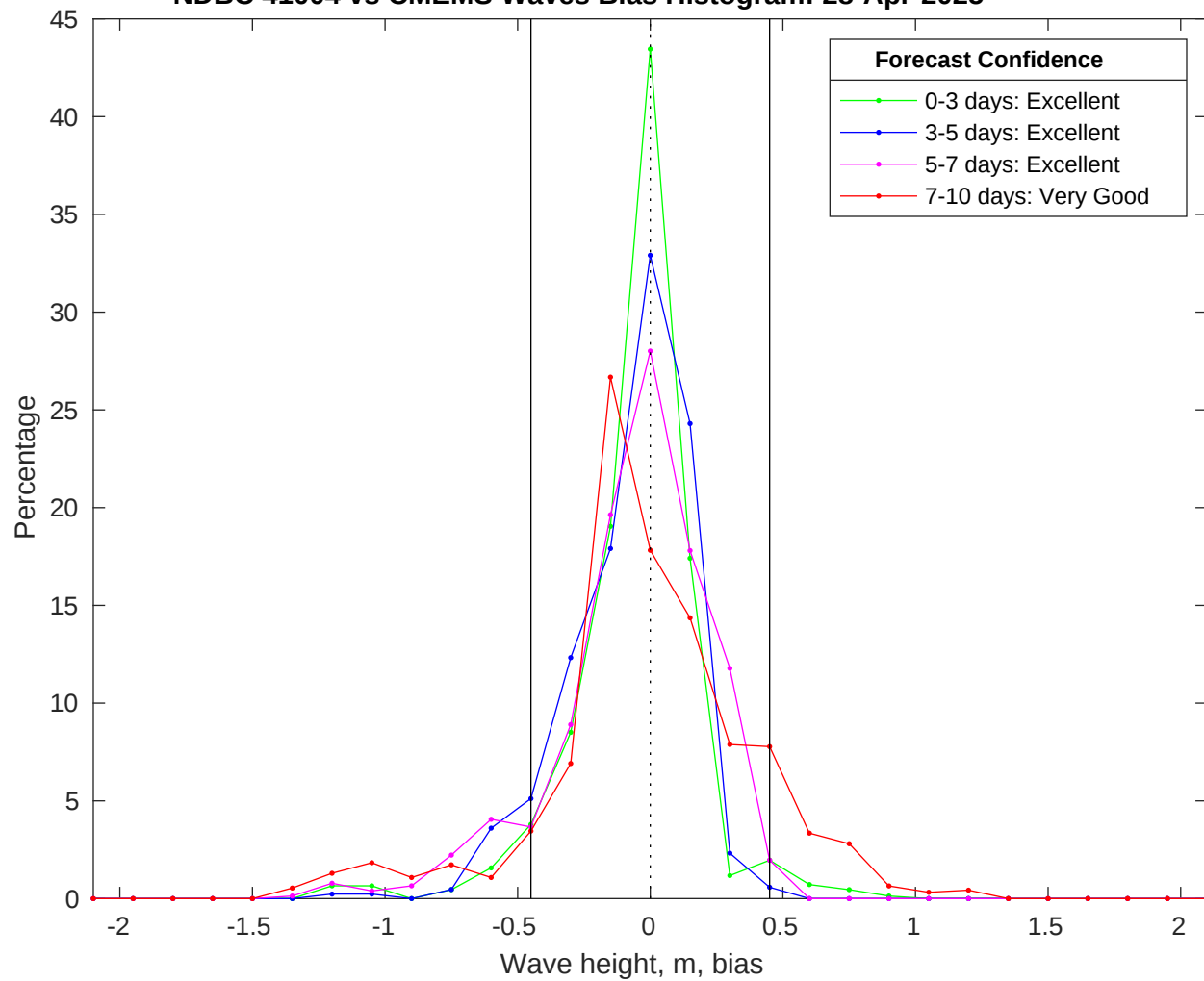
NDBC 41004 vs CMEMS Waves Bias Histogram: 28-Apr-2025
