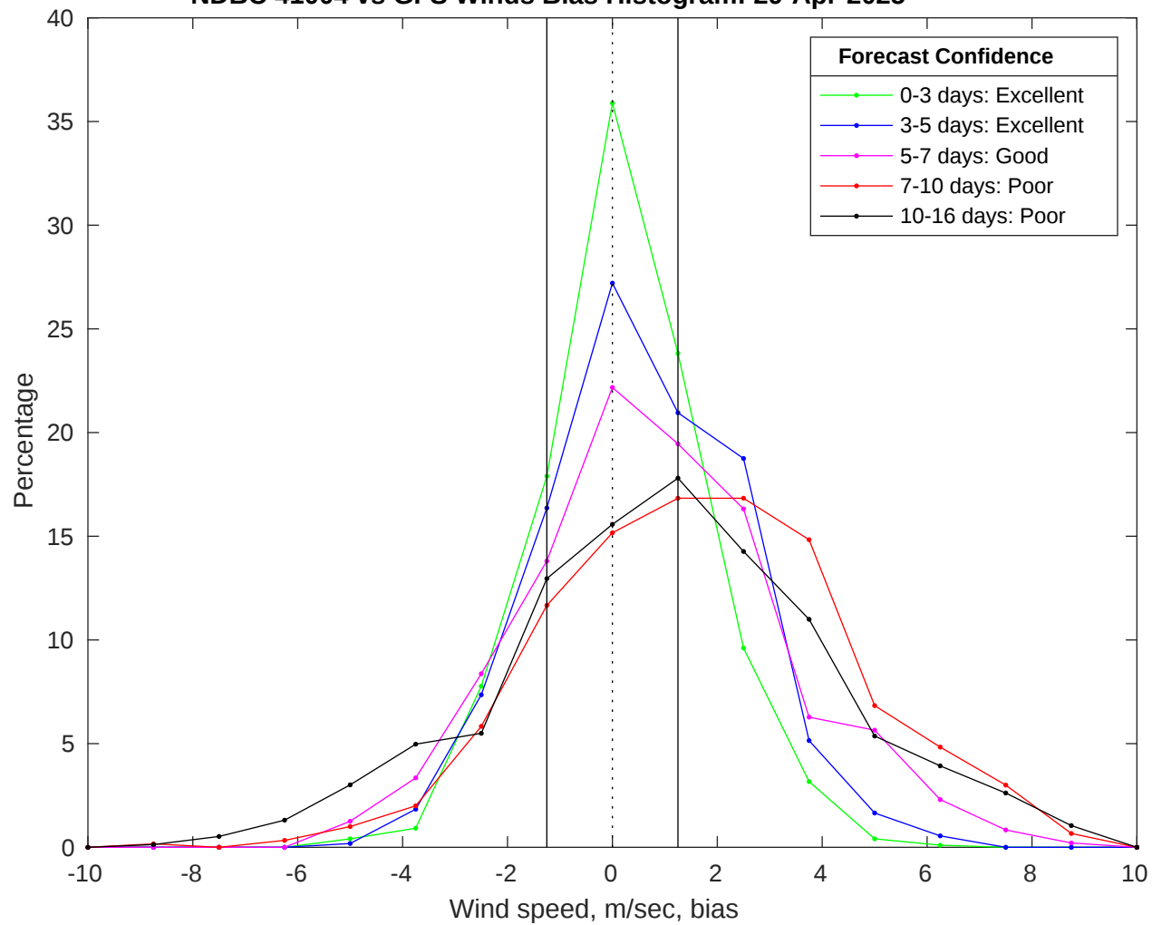
NDBC 41004 vs GFS Winds Bias Histogram: 29-Apr-2025
