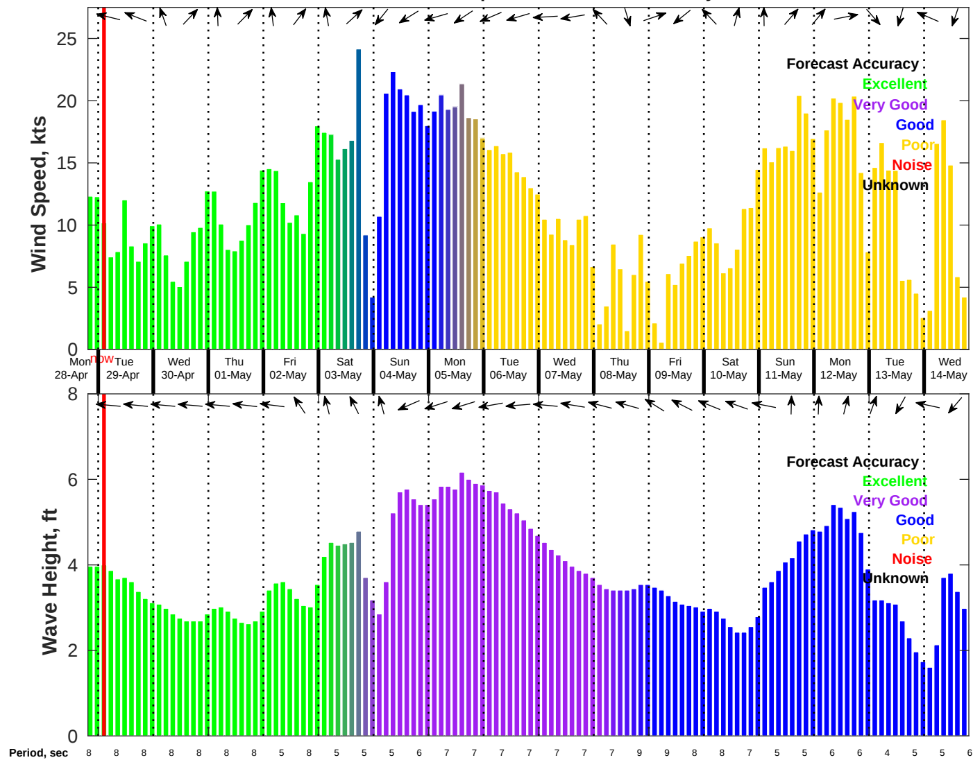
Wind & Wave Forecast for NDBC 41004 from 28-Apr-2025 19:00:00 to 14-May-2025 19:00:00
