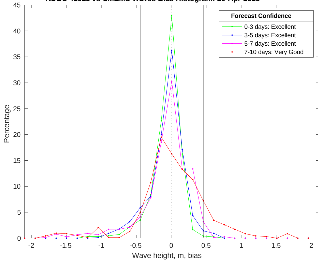
NDBC 41013 vs CMEMS Waves Bias Histogram: 29-Apr-2025
